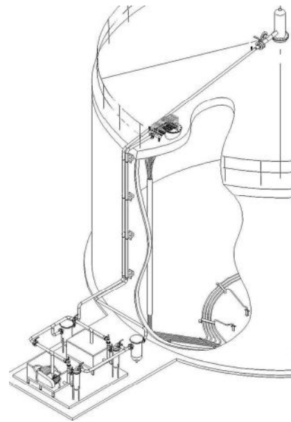
Typical Gas Mixing Layout
